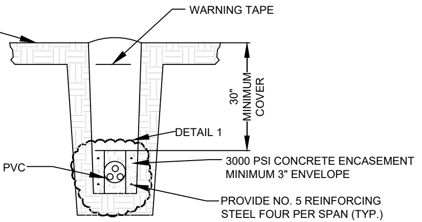
DIRECT BURIAL CONCRETE ENCASED SPLIT DUCT OPTION 1B SPANS MORE THAN 8' N.T.S.
