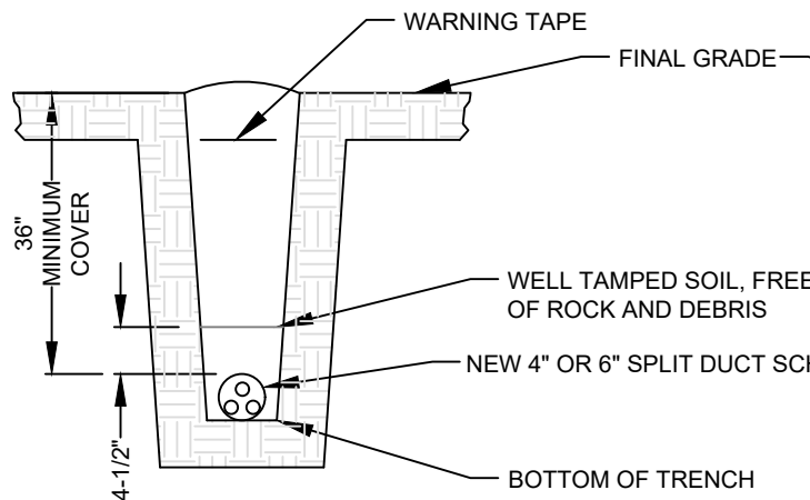
DIRECT BURIAL SPLIT DUCT OPTION 1A SPANS LESS THAN 8' N.T.S.
