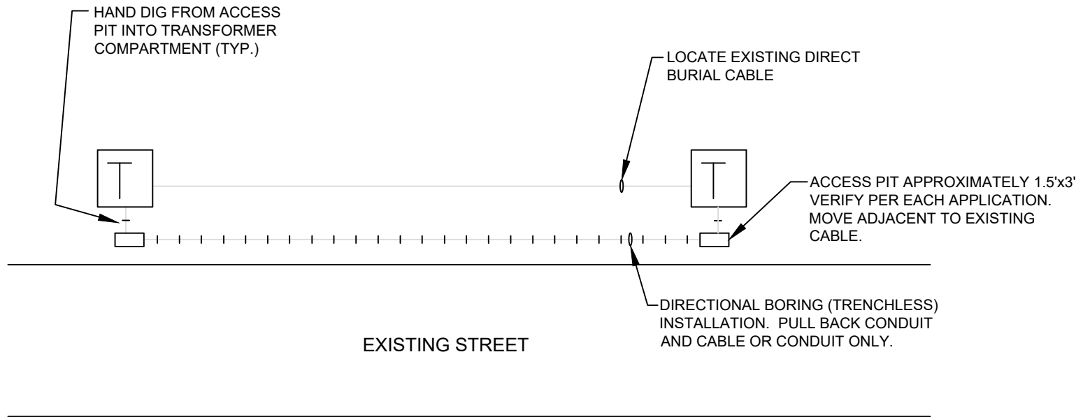
DIRECTIONAL BORING DETAIL N.T.S.
