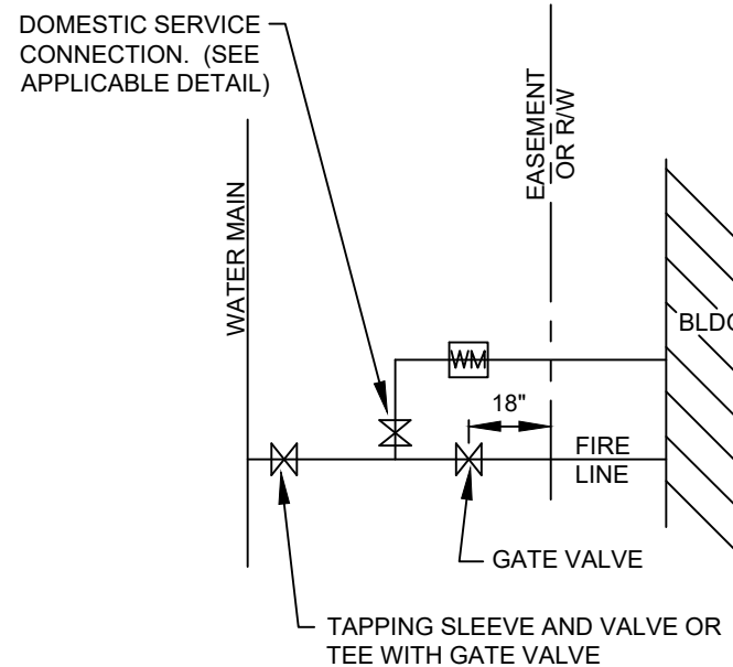
OPTIONAL FIRE LINE AND DOMESTIC SERVICE LAYOUT (AS APPROVED BY FAYPWC)
