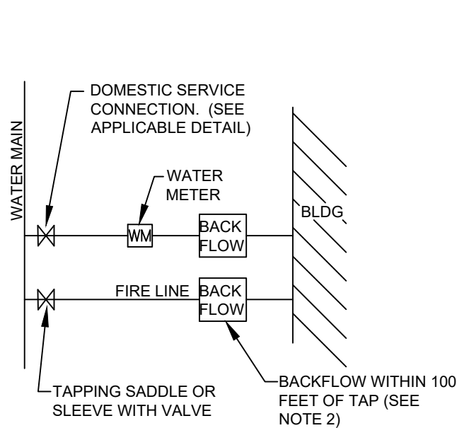
TYPICAL FIRE LINE AND DOMESTIC SERVICE LAYOUT
