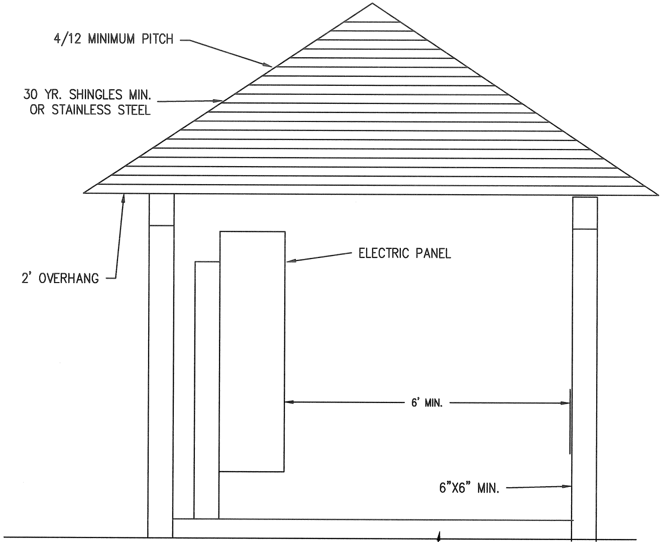
END VIEW
