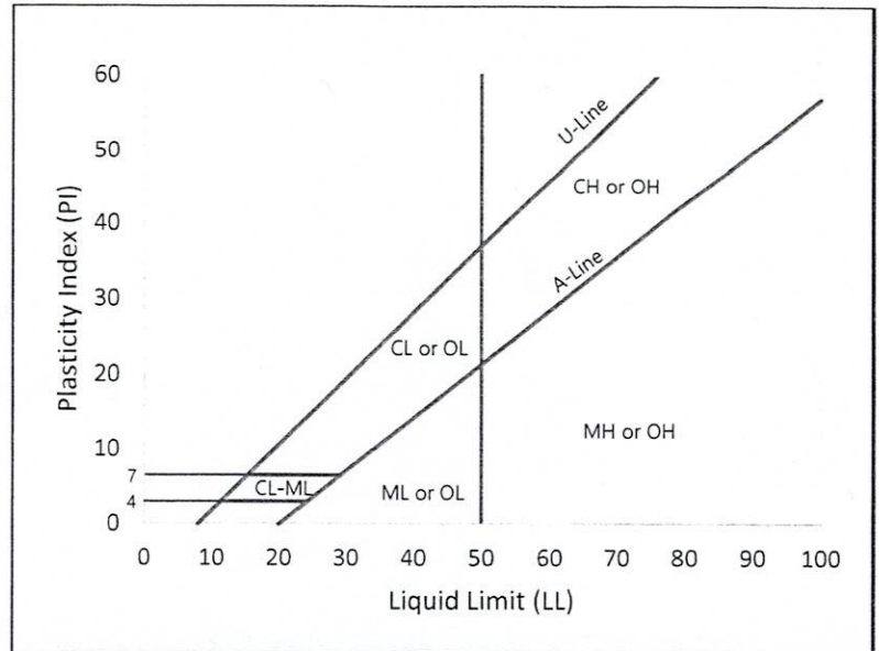
Figure 1: Plasticity Chart (based on ASTM D2487)
